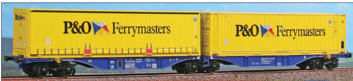
Carro intermodale Tipo Sggmrss '90 bimodulo noleggiato "P&O Ferrymasters" carico di casse mobili. Container wagon Type Sggmrss '90 hired by "P&O Ferrymasters" with swap bodies. Containerwagen Typ Sggmrss '90 Doppelmodul vermietet an "P&O Ferrymasters" mit Wechselpritschen.
